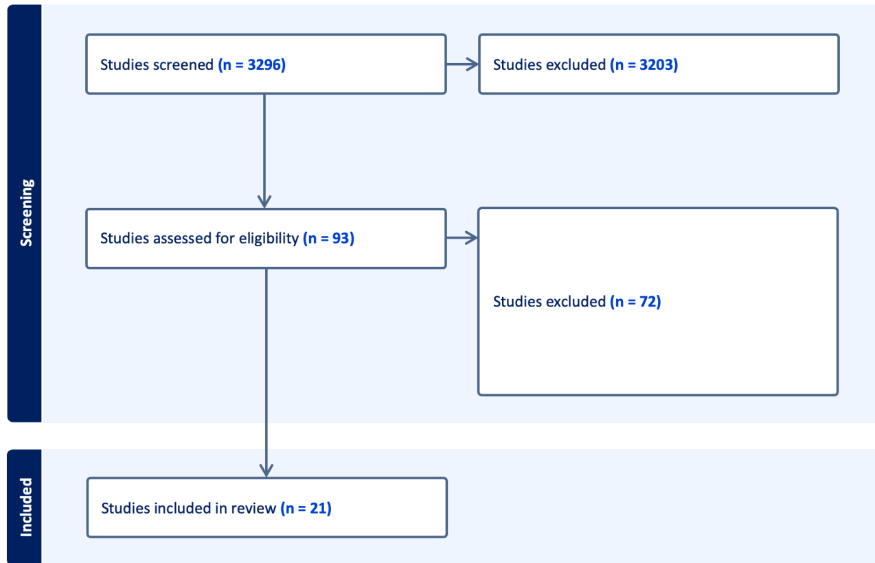
Supplementary Figure 2. PRISMA flow diagram
